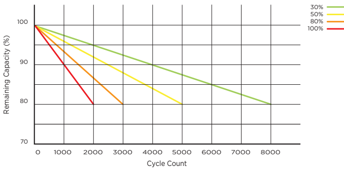
Cycle Life at Different DoD
