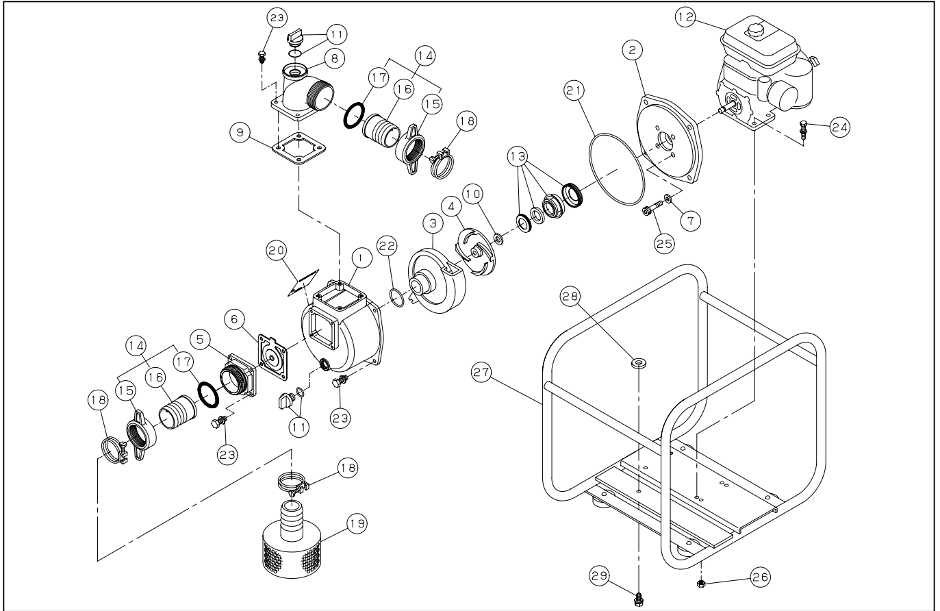
DWG No.012867603 MODEL:SEH-100X (GX240) FORM:SEH-100X-BAE-0
