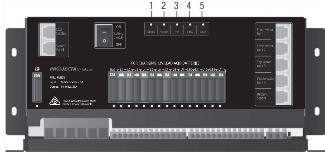
Figure 21 An overview of PM335
