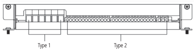
Figure 18 PM335 Terminal
