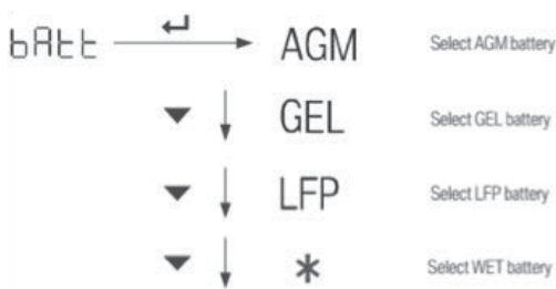
Figure 30 Battery Type setting
