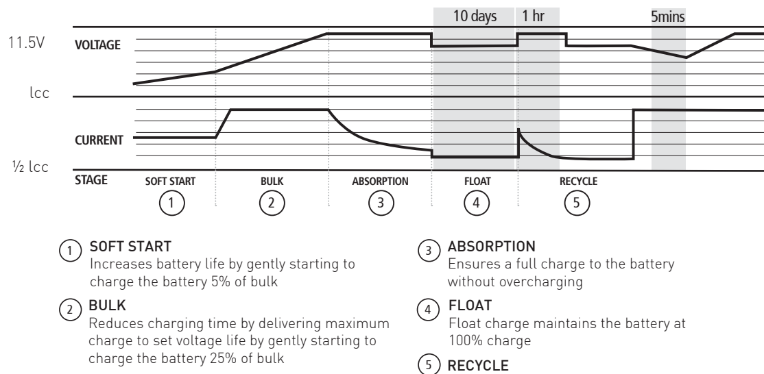
Figure 6 Charging Algorithm
