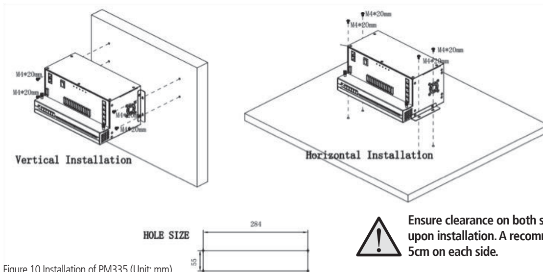
Figure 10 Installation of PM335 (Unit: mm)
