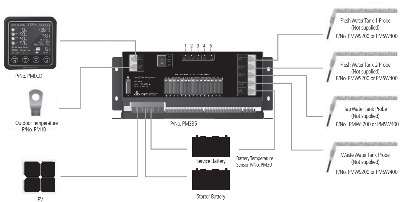
Figure 1 System Components for PM300
