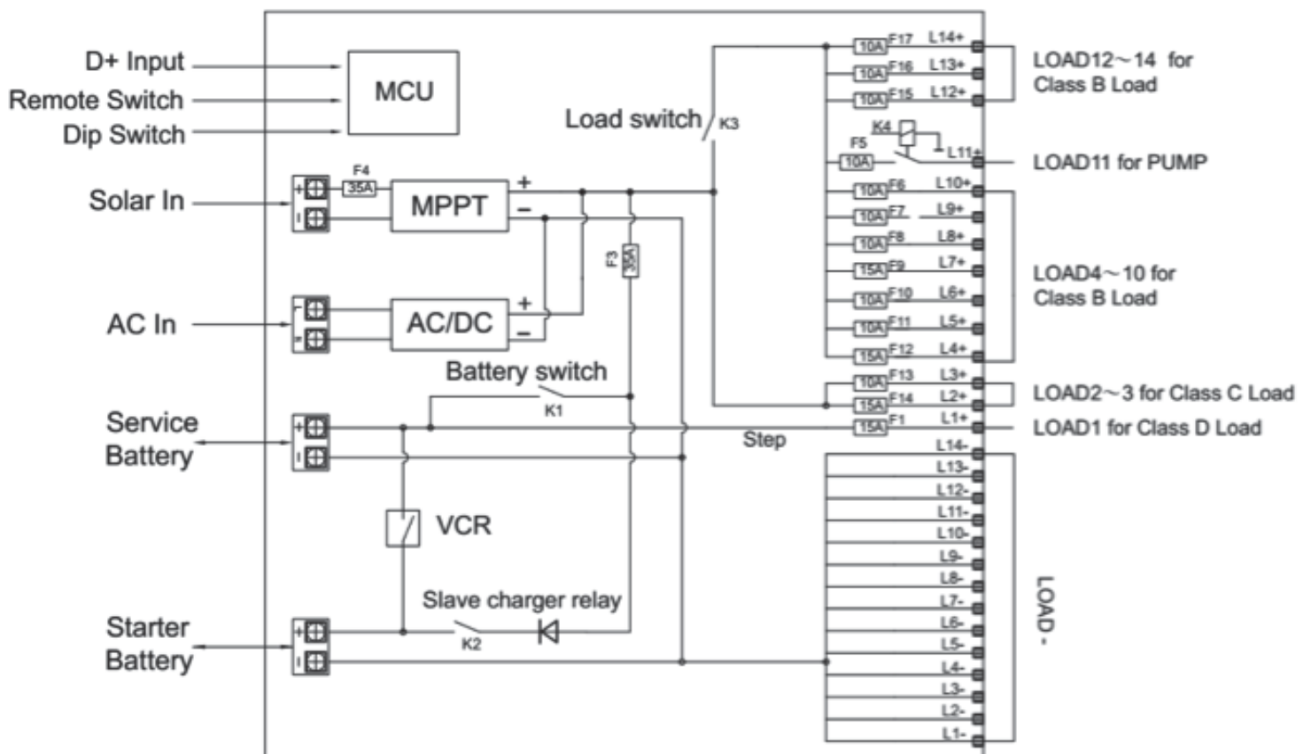
Figure 2 System Schematic
