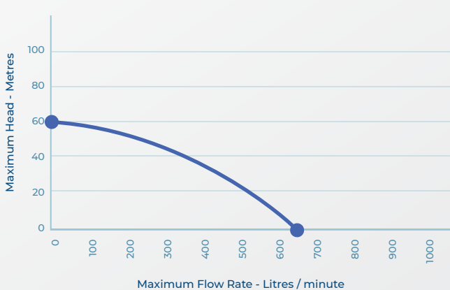
MYD15HPE PUMP PERFORMANCE CURVE
