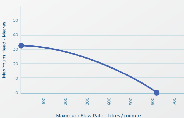
MH20-2 PUMP PERFORMANCE CURVE
