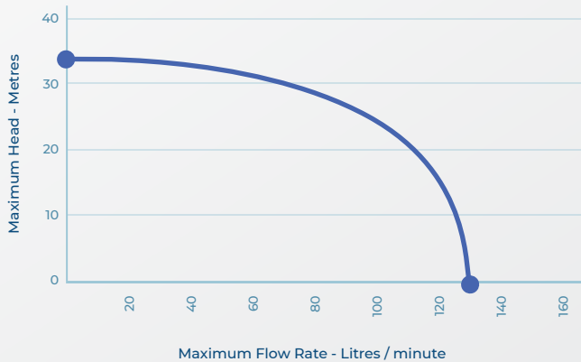
MH10-2 PUMP PERFORMANCE CURVE
