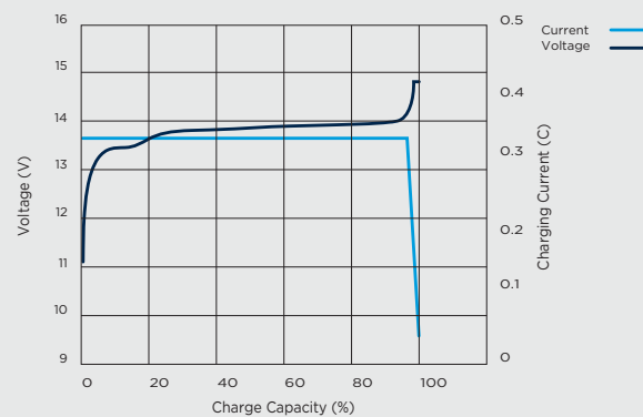
Charging Characteristic (25°C @ 0.33C)
